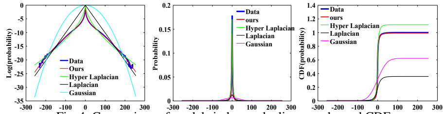
Fig. 4: Comparison of models in log scale, linear scale, and CDF.
