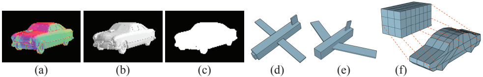
Figure 2: Lighting: Coloured directional lighting (a) provides strong cues for surface orientation; white light (b) provides less information; silhouettes (c) provide none at all. Our model is able to exploit the shading information from coloured or white lighting. Mesh parameterisations: ortho-block & full-block (assembly from cuboidal primitives, of fixed or varying orientation) are suited to objects consisting of compact parts (d-e); subdivision (per-vertex deformation of a subdivided cube) is suited to complex continuous surfaces (f).
