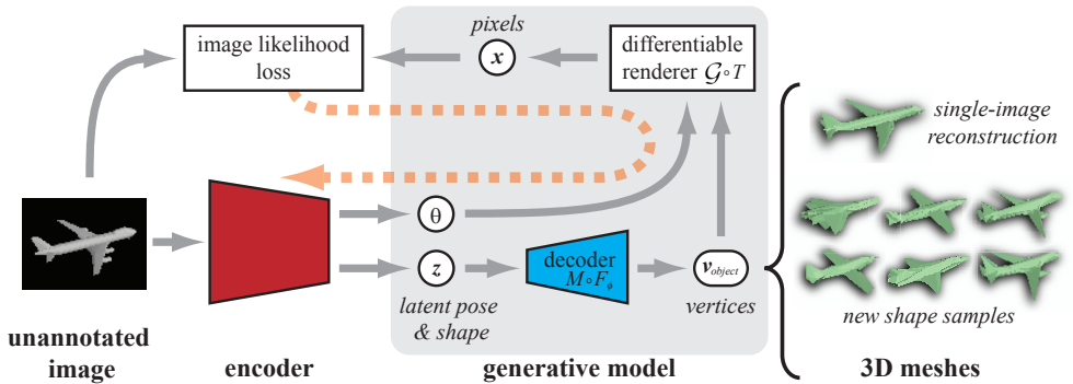
Figure 1: Given only unannotated 2D images as training data, our model learns (1) to reconstruct and predict the pose of 3D meshes from a single test image, and (2) to generate new 3D mesh samples. It is trained end-to-end (orange dashed arrow) to reconstruct input images, via a differentiable renderer that produces lit, shaded RGB images, allowing us to exploit shading cues in the loss.
