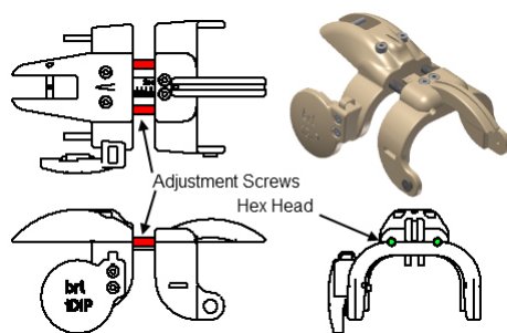
Fig. 9. The adjustment mechanism for increasing or decreasing mechanism segment lengths to fit different sized hands
