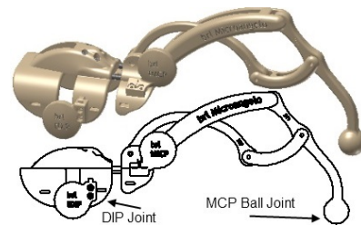
Fig. 11. Thumb MCP joint mechanism showing ball joint and four bar mechanism
