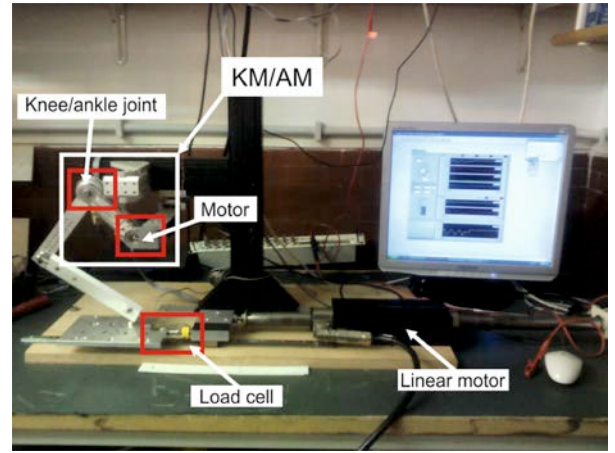
Figure 3. Experimental test bench.
