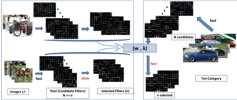
Fig. 1. Outline of our approach: Left block shows the training pipeline which is used to obtain a linear ranker (w) and diversity tradeoff parameter \lambda (described in Sect. 3) on a set of categories. Our system improves the bottleneck of the selection procedure by learning to predict the utility of filters for a new category.
