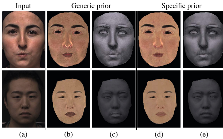
Fig. 5. Comparison between generic and specific priors. (a) Input image. (b/d) Estimated reflectance. (c/e) Estimated shading.
