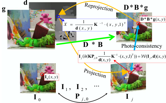
Figure 1. The relationship between the low-resolution input sequence \mathbf{I}_j and the super-resolution image \mathbf{g} , induced by the depth map \mathbf{d} : The photometric consistency should hold for \mathbf{I}_j and the simulated low-resolution image \mathbf{D} * \mathbf{B} * \mathbf{g} .
