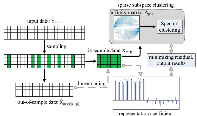
Figure 1. Architecture of our Scalable Sparse Subspace Clustering algorithm.
