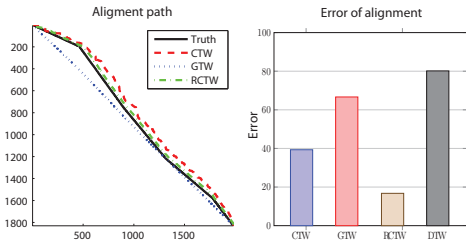
Figure 3. Comparison of the performance of the CTW, the GTW, and the RCTW on synthetic data alignment. The mean alignment path (left) and the mean alignment error (right) obtained by the CTW, the GTW, and the RCTW (left) by applying 50 different random spatial and temporal transformations on the latent data sequence \mathbf{Z} .
