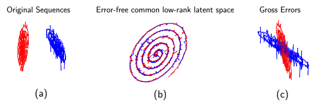
Figure 1. The RCTW applied on grossly-corrupted 3D data. (a) Original grossly-corrupted 3D data. (b) Alignment of the two data sequences onto an error-free common low-rank latent subspace which has been robustly estimated by the RCTW. (c) The removed gross errors.
