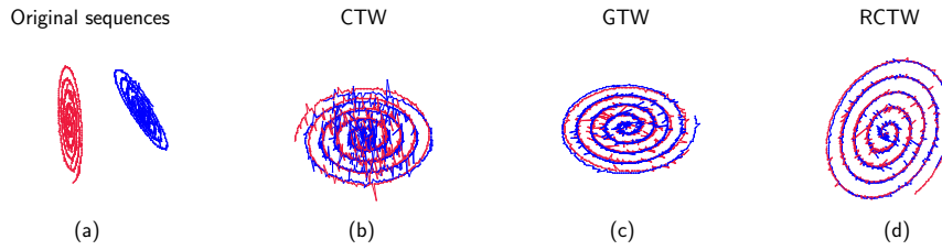
Figure 2. Alignment of synthetic data; 30% of the samples of each sequence have been contaminated by gross errors. (a) Initial noisy data sequences. The alignment achieved by (b) the CTW, (c) the GTW, and (d) the RCTW.
