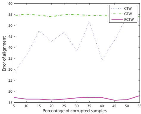
Figure 4. Mean alignment error obtained by the CTW, the GTW, and the RCTW, as a function of the percentage of corrupted samples on synthetic data sequences.
