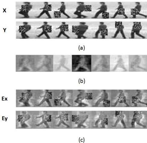
Figure 6. Alignment of occluded human walking sequences obtained by the RCTW. (a) The initial occluded walking sequences i.e., \mathbf{X} , \mathbf{Y} . (b) Aligned sequences onto the error-free latent common space which has been robustly estimated by the RCTW. (c) Magnitude of the recovered gross errors.
