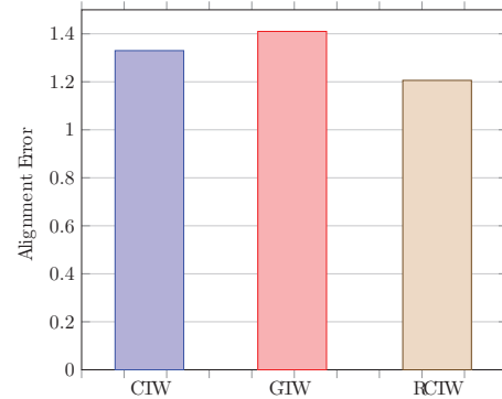
Figure 5. Mean alignment error obtained by the CTW, the GTW and the RCTW on human walking sequences by the KTH.
