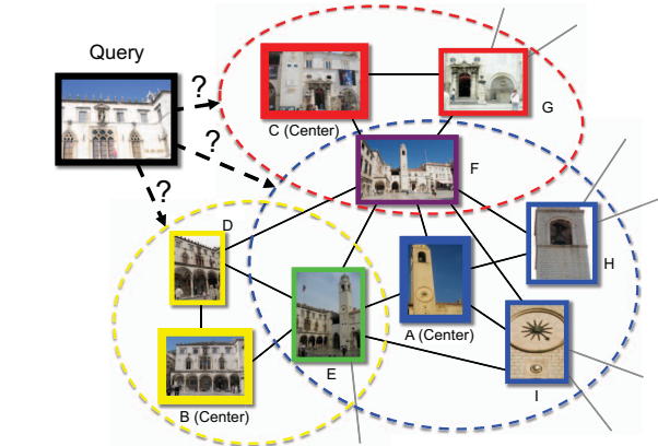
Figure 1. A segment of an example image matching graph with three clusters defined by representative images A, B and C. Nodes in this graph are images, and edge connect overlapping images. In order to match a new query image to the graph, our method learns local distance functions for a set of neighborhoods that cover the graph, for instance, the neighborhoods centered at nodes A, B, and C, circled with colored boundaries. Given a query image, we match to the graph using these learned neighborhood models, rather than considering database images individually. Each neighborhood has its own distinctive features, and our goal is to learn and use them to aid recognition.
