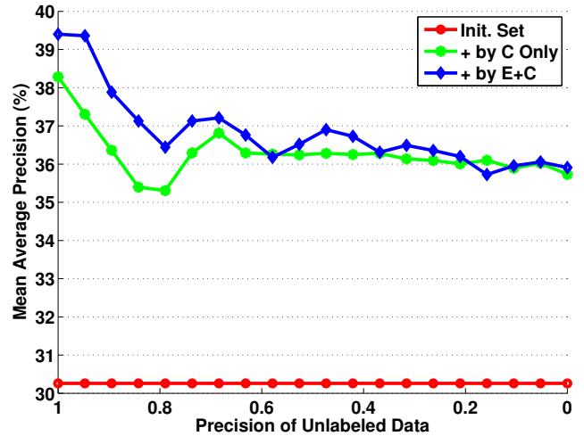
Figure 6. Mean average precision (mAP) as a function of precision of unlabeled data. Precision denotes the ratio of size of the unlabeled images from extraneous categories to the size of the entire unlabeled image data (size = 50,000). Although precision decreases, the mean average precisions (mAP) by our method do not decrease much.
