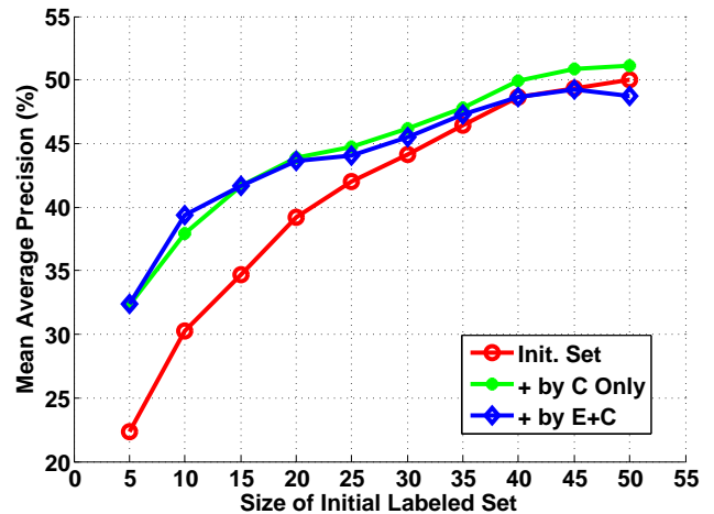
Figure 7. Mean average precision (mAP) as a function of the size of the initial labeled set. The number of added samples is 50 in all experiments.
