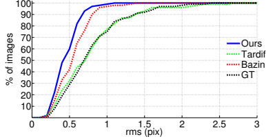
Figure 6. Cumulative consistency error computed using our D for the three groups of ground truth edges (belonging to orthogonal VDs). For each image we compute the root-mean-square (rms) consistency error across all lines fitting the estimated VPs; GT corresponds to the ground truth VPs provided by YUD.
