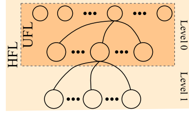
Figure 2. A HFL problem with two layers is shown. The first layer l = 0 corresponds to the UFL problem, where the customers e_i need to be served by the facilities \mathbf{v}_j^0 . The second layer l = 1 contains the storage facilities \mathbf{v}_k^1 that are the suppliers of \mathbf{v}_j^0 .
