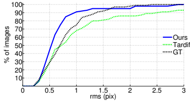
Figure 7. Cumulative consistency error computed using D for the three groups of ground truth edges. The results for Ours and Tardif were obtained using edges automatically detected.
