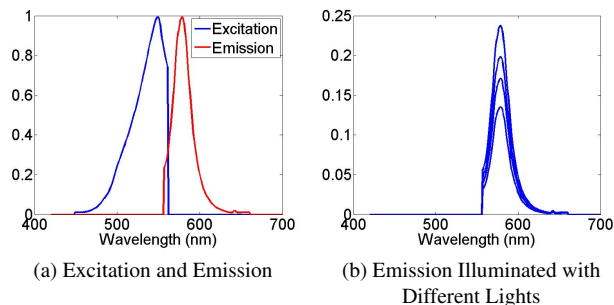
Figure 2: Sample Excitation and Emission Spectra
