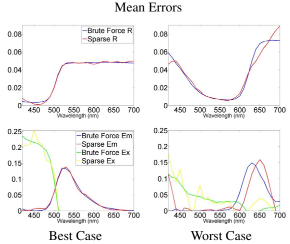
Figure 4: Brute force versus sparse wavelength imaging of spectra on color charts. Despite the worst case having a poorly estimated Ex we found that the error had little effect on relighting performance. The mean errors between sparse wavelength and brute force imaging are shown at the top.
