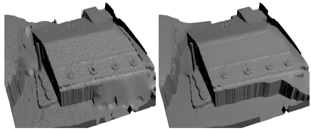
Figure 1. The depth map fusion result of a stack of depth maps is shown as a 3D rendering. Total generalized variation regularization used for the fusion has the property to favor piecewise affine functions like the roof or the street. However, there is a trade-off between affine pieces and discontinuities. For convex \ell_1 -norm regularization ( left ) this trade-off is rather sensible. This paper enables the optimization of non-convex norms ( right ) which emphasize the model properties and perform better for many computer vision tasks.
