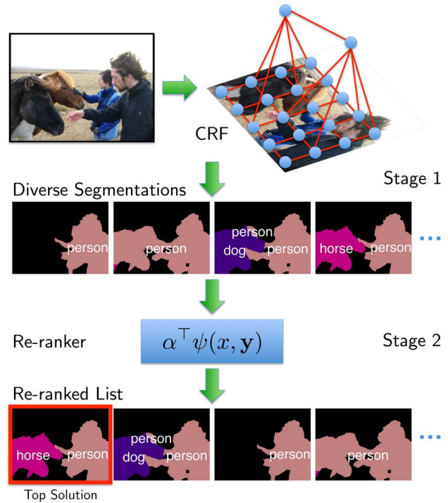
Figure 1: An overview of our DivMBEST+RERANK approach. In Stage 1 diverse segmentations are computed from a tractable probabilistic model. These are fed to a large-margin re-ranker in Stage 2 . The top re-ranked segmentation is returned as the final solution. Even though the most probable segmentation from Stage 1 is incorrect, the set of segmentations does contain an accurate solution, which the re-ranker is able to score to the top.
