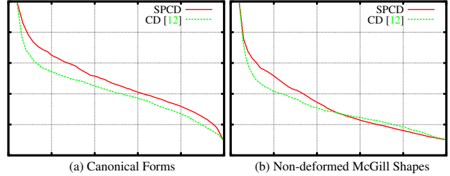
Figure 7. Average Precision-Recall curves on the canonical forms (a) and the non-deformed (b) shapes of the first 10 classes of the McGill Shape Benchmark. The average precision ( y -axis) is higher on the less diverse classes of the canonical forms than on the non-deformed McGill shapes. The precision of SPCD (red) is higher on both data sets at low recall rates.
