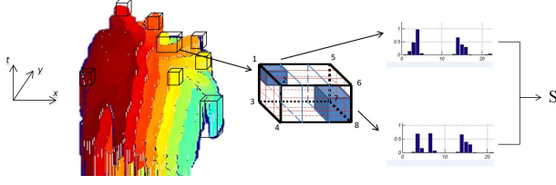
Figure 3: Illustration of extracting DCSF from depth video
