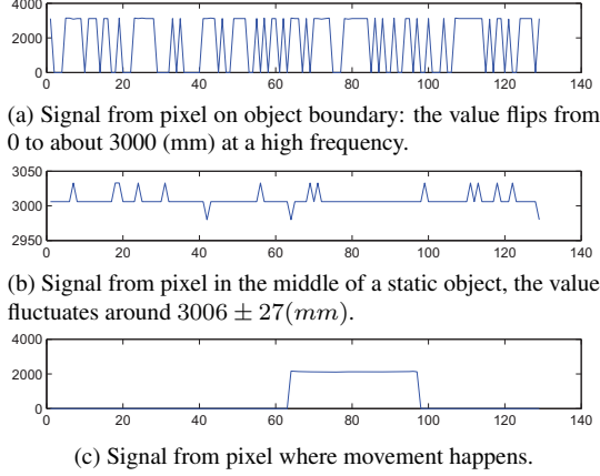
Figure 1: Temporal evolution of pixel values at different locations in the scene.
