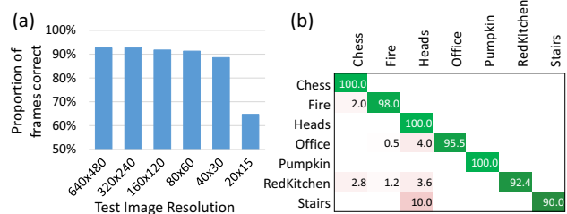
Figure 5. (a) Effect of image resolution on accuracy for DA-RGB Chess. (b) Scene recognition confusion matrix. For Chess, Heads, and Pumpkin we achieve correct recognition for all test frames.
