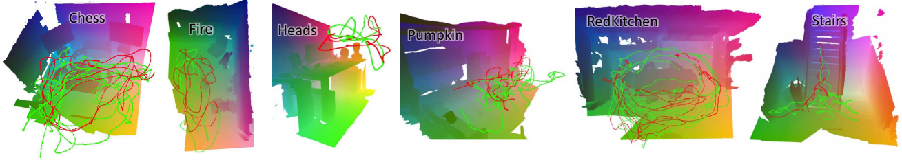
Figure 3. The 7 Scenes dataset. These renderings show the scene coordinate representations for each scene as RGB colors. The green and red camera tracks show the positions of the cameras in the training and test sequences. The Office scene is shown in Fig. 1.
