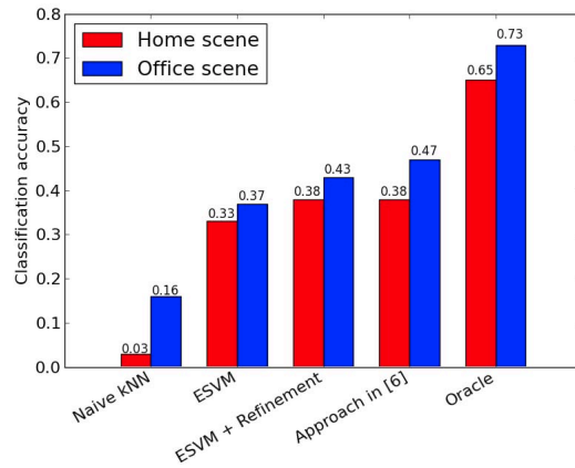
Figure 6. Point cloud labeling accuracy of different baselines in both office and home scenes.
