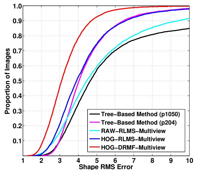
Figure 2. Experiment on Multi-PIE database.
