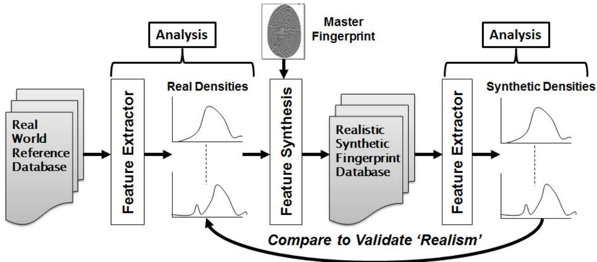
Figure 1: Analysis-by-synthesis process for synthetic fingerprint generation.
