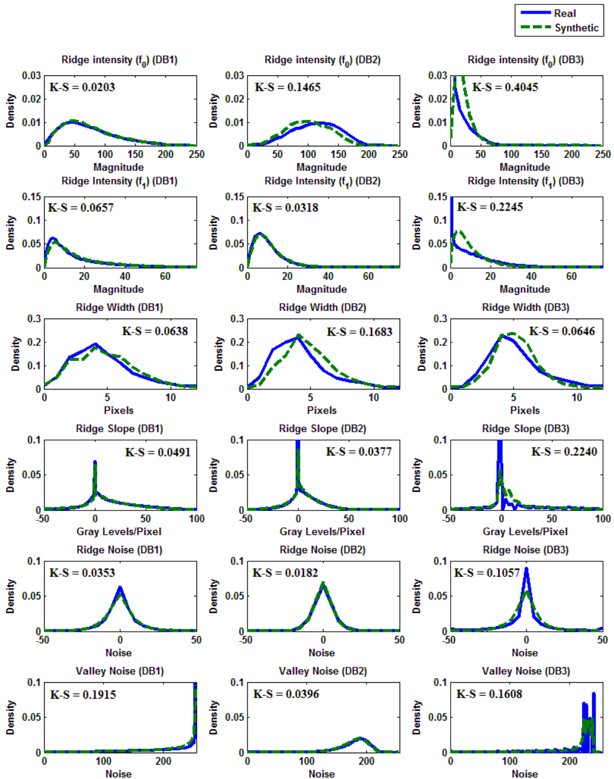
Figure 3: Comparison of real and synthetic feature distributions measured from 800 real fingerprint images from each of the three real FVC2004 databases and 800 synthetic fingerprint images representative of each of the real databases in terms of texture. Distributions are compared using the two-sample Kolmogorov-Smirnov (K-S) test and each K-S statistic is reported.
