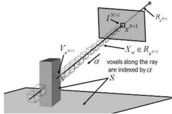
Figure 3 The interaction of a ray with the cells in the volume for probabilistic inference such as rendering image.
