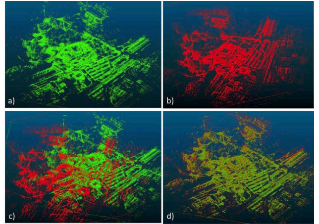
Figure 5 3-d to 3-d registration by aligning the 3-d point clouds. a) and b) point clouds obtained from dense volumetric 3-d models for EO and IR imagery, respectively. c) initial alignment of the two point clouds and d) accurate alignment after applying [7], [9].
