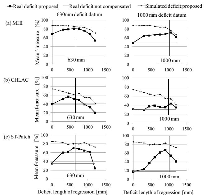
Figure 12: Evaluation results of actual deficient datum.
