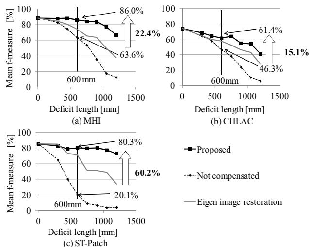
Figure 11: Evaluation results of simulated deficient datum.
