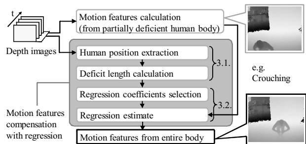
Figure 1: Outline of motion features compensation.
