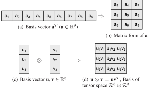
Figure 1. Take face images of size 3 \times 3 . The ordinary vector-based subspace learning algorithms (e.g. PCA and LDA) first convert the face images to 9-dimensional vectors and compute the basis vectors (projection functions). The basis vector is also 9-dimensional, as shown in (a). (b) The basis vector can be converted to the matrix form and shown as an image, which was referred as Eigenface (PCA) and Fisherface (LDA). The 9 numbers in the basis vector are independent estimated and there is no spatial relation between them. (c) The tensor-based subspace learning approaches directly take 3 \times 3 face images as input and compute a set of 3-dimensional basis vectors \mathbf{u} 's and \mathbf{v} 's. (d) Each \mathbf{u} and \mathbf{v} form a basis \mathbf{u} \otimes \mathbf{v} in tensor space which can also be shown as an image. The 9 numbers in the tensor basis only have 6 degrees of freedom and the values in the same row (column) have a common divisor. However, there is no guarantee of the spatial smoothness of the basis function.
