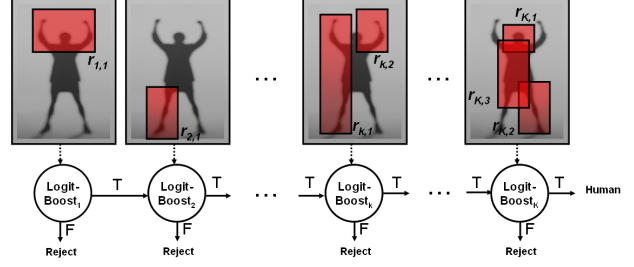
Figure 3. Cascade of LogitBoost classifiers. The k th LogitBoost classifier selects normalized covariance descriptors of subwindows r_{k,i} .
