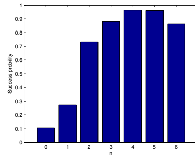
Figure 4. Probability of success with different order n of the robust estimator function.
