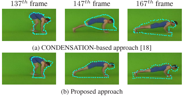
Figure 6. Tracking results on a video sequence: (a) CONDENSATION-based approach with uniform transition probability, (b) proposed approach which can track without knowing transition probabilities. (a) gets back to track after 30 frames, while our approach is able to maintain tracking continuously.
