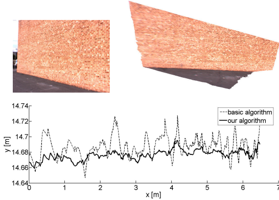
Figure 5. Comparison of the basic fronto-parallel plane sweep and sweeping in multiple directions. Top left : the original view-point. Top right : The depthmap triangulated into a polygonal mesh viewed from above. Bottom : A cross-section of the surface. Note the scale on the axes. We measured the standard deviation of the surface from the best-fit line. This was 1.31 cm for the fronto-parallel sweep and 0.61 cm for our algorithm.
