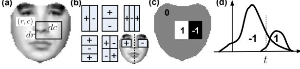
Figure 3. (a) The parametrization of a weak classifier; (b) The six feature types; (c) The notional template \mathbf{A} , whose inner product with the warped image is mathematically equivalent to computing a rectangular feature; (d) Let the rectangular features of the positive samples have larger mean than that of the negative samples, by multiplying a sign g = \{1, -1\} , and then estimate the threshold t that has the minimal weighted LS error via binary search.
