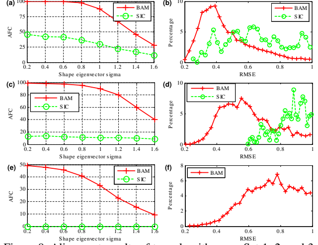
Figure 9. Alignment results of two algorithms on Set 1, 2, and 3. From top to bottom, each row is the result for one set. Left column is the AFC; right column is the histogram of the resultant RMSE for the trials where both algorithms converge. Only the HRMSE of the BAM is plotted at (f) since the SIC has no convergence.
