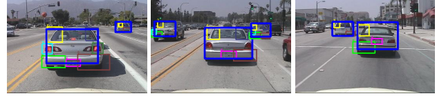
Figure 8. Car rear detection results with optimal (4, 3) covering ensemble and corresponding parts.
