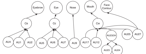
Figure 3. The relationship between the AUs and the local facial component shape. Intermediate nodes ( C_B , C_E , and C_M ) are introduced to model the correlations among AUs.
