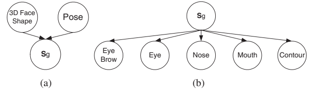
Figure 2. (a) The head pose and 3D facial shape directly affect the 2D global shape S_g . (b) The causal relationship between the global shape S_g and the local facial component shapes.
