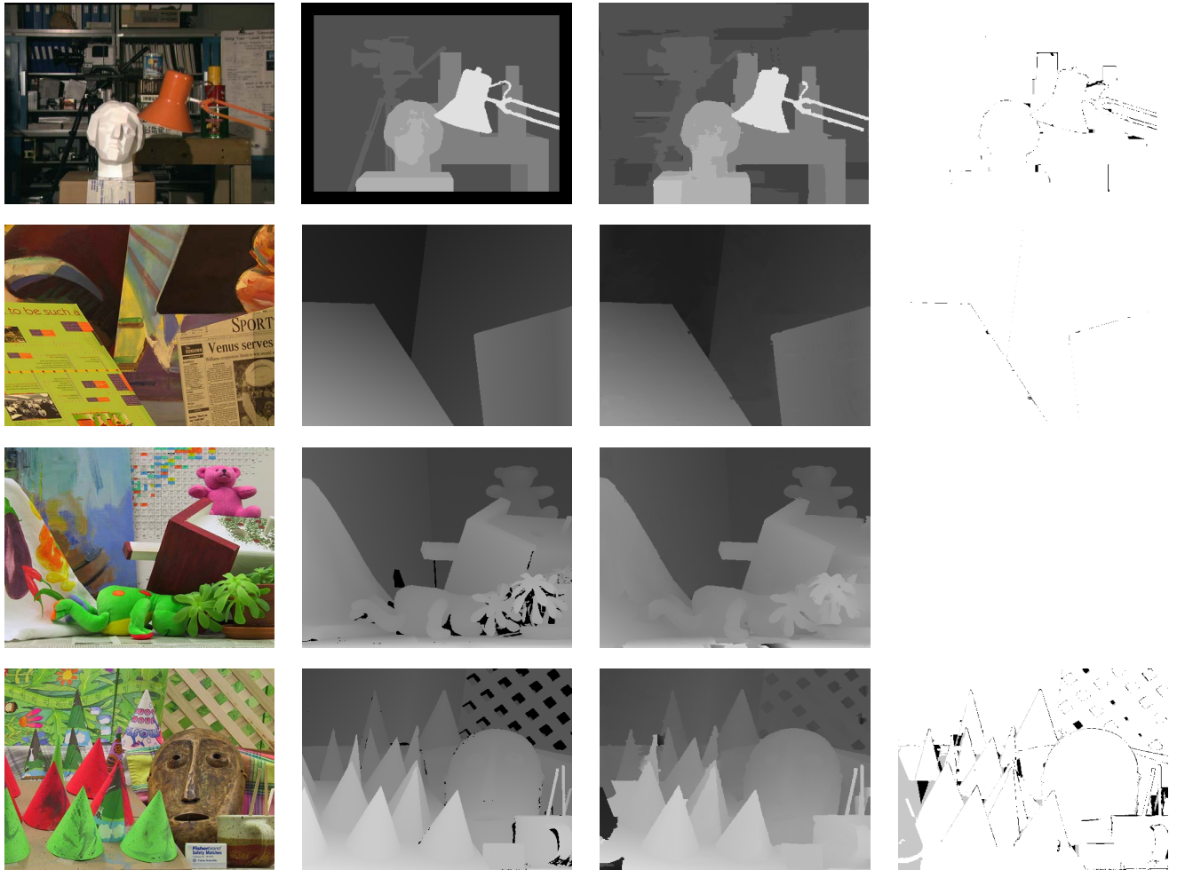
Figure 9 The disparity maps of the standard stereo image pairs on Middleburry website obtain by our algorithm: The 1 st row – Tsukuba, the 2 nd row- Venus, the 3 rd –Teddy, and the 4 th –Cones The 1 st column – reference image, the 2 nd column – ground truth, the 3 rd column – our algorithm, and the 4 th column – matching errors.
