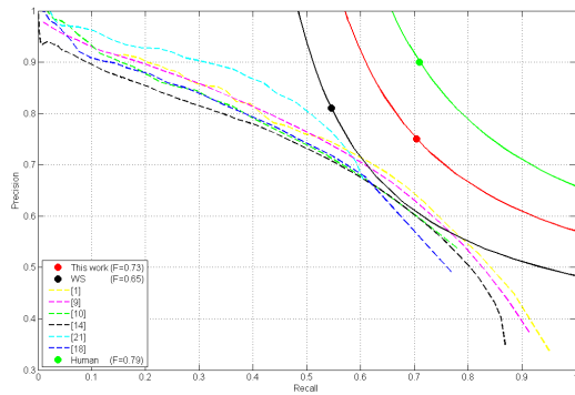
Figure 7. Benchmark Results
