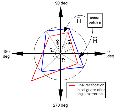
Figure 2. A first estimate of the patch transformation is obtained using a classifier that provides the values of the angles a_i defined as the angles between the lines that go through the patch center and each of the four corners.
