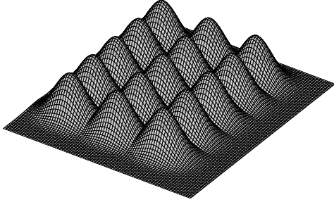
(b) Tensor product B-spline
