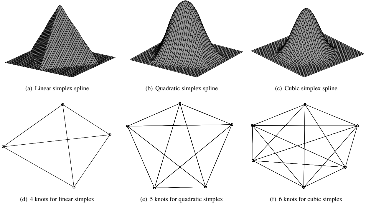
Figure 2. Simplex splines of increasing order and smoothness.
