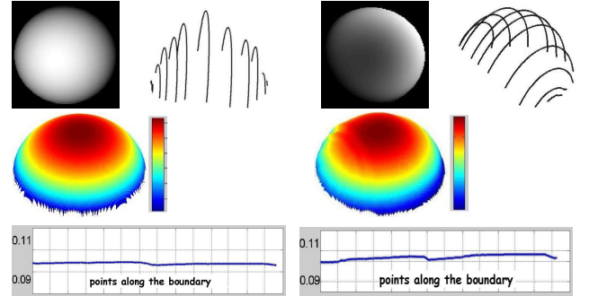
Figure 3. Reconstruction of a synthetic sphere with uniform (left) and non-uniform smooth (right) albedo. Light directions are [-0.3, 0.2, 0.93] and [0.5, -0.3, 0.8] respectively. Top: an image used for reconstruction (one of two in the case of the non-uniform albedo) and characteristic curves; Second row: 3D reconstruction with a characteristics solution; Bottom: recovered depth along the boundary.
