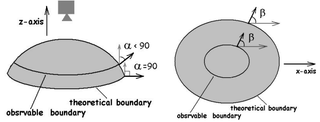
Figure 2. Computing boundary conditions. The figure shows a surface (left) viewed from above (right). The rim of the surface forms the “theoretical boundary,” but intensities are only visible in internal points. We assume that by moving within the image into the inside of the shape we reach surface points whose normal is coplanar with their respective point on the rim.
