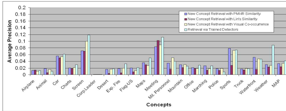
Figure 4. A comparison of different retrieval methods using Average Precision. MAP (Mean Average Precision) is shown at far right.
