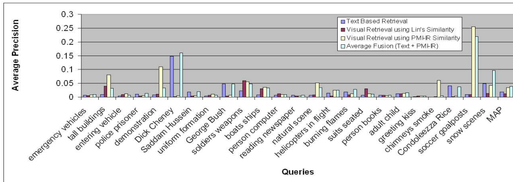
Figure 8. AP (Average Precision) results for different semantic retrieval methods for each query (represented by some selected words for each query) in TRECVID'06. MAP (Mean Average Precision) is shown at far right.
