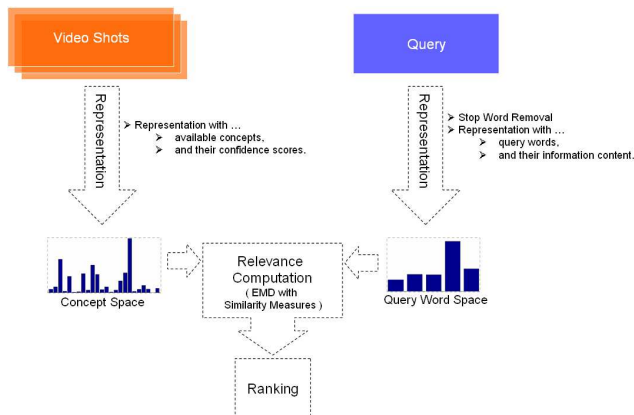
Figure 2. An overview of the Visual Content-based Semantic Video Retrieval method.
