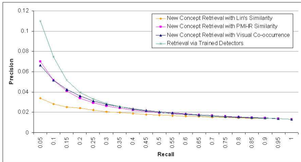
Figure 7. Average precision-recall curves for different concept retrieval methods.
