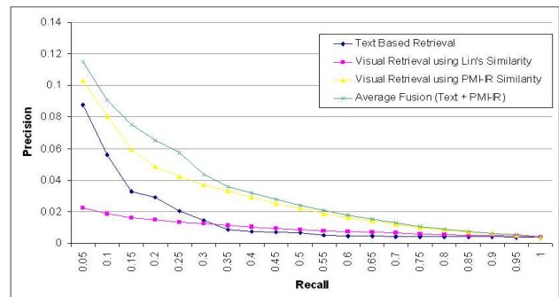
Figure 9. Average precision-recall curves for different semantic retrieval methods on TRECVID'06 queries.
