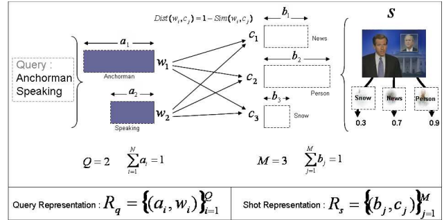
Figure 3. EMD based distance computation between the visual content and the query.
