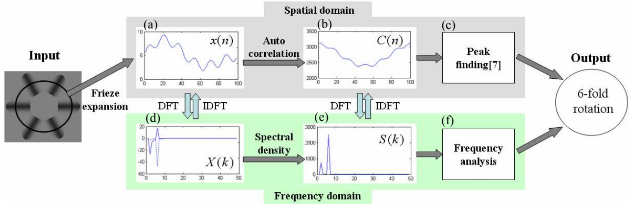
Figure 5: Relation between spectral density S(k) and autocorrelation C(n) . ((a)->(d)->(e)->(f)) is the processes of our algorithm, which is equivalent to using the DFT of autocorrelation ((a)->(b)->(e)->(f)). Peak finding algorithms [7] use (a)->(d)->(e)->(b)->(c) to reduce the time complexity. * DC coefficients are not shown.
