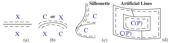
Figure 2. Illustration of Properties 1–4. (a) A straight edge. (b) A curved edge. (c) A silhouette. (d) Two faces connected by two artificial lines.
