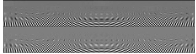
Figure 2. Gabor kernels with 5 scales and 36 orientations: real part kernels (rows 1 to 5) and imaginary part kernels (rows 6 to 10).
