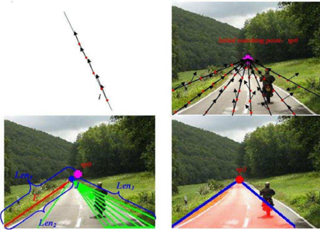
Figure 7. Illustration of detection of the two most dominant edges. Top left: line segments consisting of discrete oriented points. Top right: initially detected vanishing point. Bottom left: detection of the two most dominant edges based on initial vanishing point. Bottom right: the two most dominant edges and updated vanishing point.
