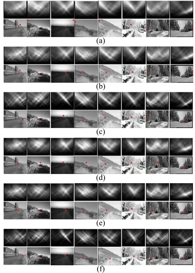
Figure 8. Comparison of vanishing point estimation based on different combinations.
