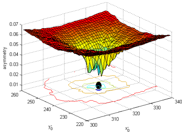
Figure 5. Profile of asymmetry measure with respect to different hypothesized positions of the optical center (x_0, y_0) for the image in Fig. 2. The true optical center is marked by the black circle.
