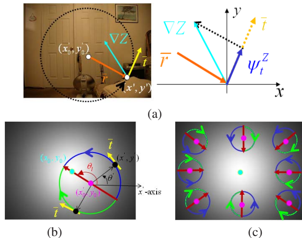
Figure 1. Illustration of semicircular tangential gradients (SCTG). (a) Counterclockwise SCTG. (b) Assignment of clockwise or counterclockwise SCTGs. (c) Effect of estimated optical center on SCTG assignment using Eq. (6), where the pink dots are different optical center estimates and the light blue dot is the true optical center.
