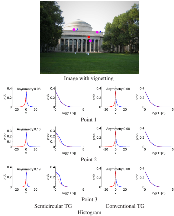
Figure 2. Comparison of semicircular tangential gradient (SCTG) and conventional TG distributions. The true optical center and three estimated optical centers are marked by the red dot and three purple dots, respectively. With each distribution, a \log(1 + |x|) histogram is also shown to emphasize asymmetry.
