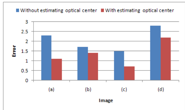
Figure 8. Mean Squared Errors ( \times 10^{-3} ) in the vignetting function estimated by the method in [20], with and without optical center estimation by our proposed method.
