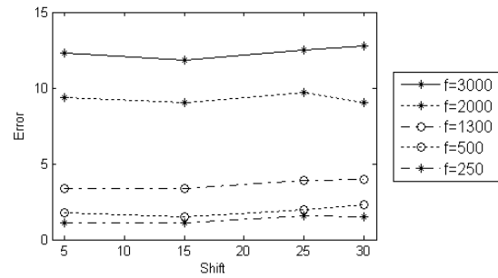
Figure 6. Errors in optical center estimation using images with simulated vignetting. The vignetting effects are simulated with different focal lengths f and random shifts of the optical center away from the numerical center of the image coordinates.
