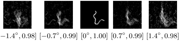
Figure 2. The images in the top row are the blur kernel estimated using the blurred image (b) and a number of clear images (a) after a small alignment perturbation of different rotation and scale. Two numbers in brackets under each kernel are the rotation angle and scale value (\theta, s) . All images are from [20].
