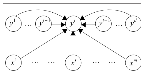
Figure 1. Dependency model for one output variable of SOAR. y^t is the current output, and m and d are dimensionality of inputs and outputs, respectively. Notice y^t not only depends on the input \mathbf{x} = [x^1, \dots, x^m]^\top , but also on the remaining outputs \mathbf{y}^{-t} = \mathbf{y} \setminus y^t .
