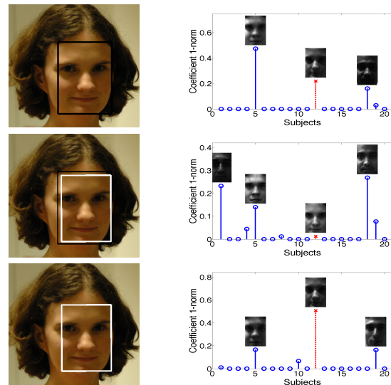
Figure 1. Compound effect of registration and illumination.
