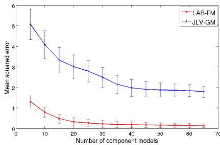
Figure 11. The performance comparison on weather data.
