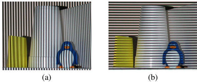
Figure 1. The frequency of observed patterns is sensitive to the geometry of the scene. (a) Vertical stripes projected from a projector placed at the left hand side of the camera. Notice the different frequencies on the two slanted planes (left and right), and curved lines on the penguin; (b) By projecting horizontal stripes, the frequency of the observed patterns is geometry-invariant.
