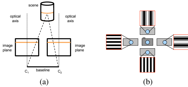
Figure 2. Geometry of the capture setup. (a) correspondence between epipolar lines in the canonical stereo configuration, considering perspective cameras; (b) sample configuration with a camera and four projectors; (c) experimental table-top prototype; (d) the scene being imaged.
