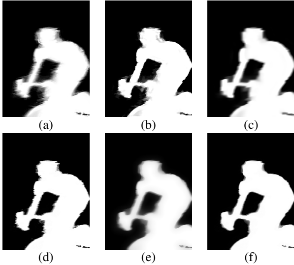
Figure 5. Comparison of \alpha estimation algorithms given \alpha_p and p (the estimated motion vector is (14, -3)' ), (a) noisy \alpha_p extracted by the matting algorithm, (b) result by the back-projection method [13], (c) result by deconvolution with sparsity prior [17], (d) our result without the edge smoothness prior term, (e) our result without the binary prior term, (f) result by our method (Eqn. 13).
