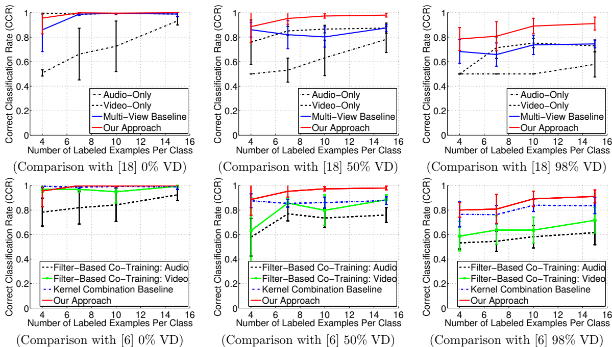
Figure 4. Audio-visual recognition with varying training set sizes: Classification accuracy as a function of the number of training samples for 0%, 50% and 98% view disagreement. Performance is shown averaged across 10 splits, the error bars indicate \pm 1 std. deviation. (top) Comparison with single-view and Bayesian co-training approaches, and (bottom) audio and video classifiers from filter-based co-training [6] and the results of multi-view GP kernel combination (see text for details). In contrast to the baseline approaches, our method is able successfully combine each view to achieve good classification accuracy even in the presence of gross view corruption (98% view disagreement).
