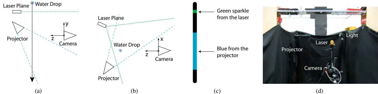
Figure 2. A side view (a) and top view (b) of a water drop as it crosses the laser plane and projector field of view. The image generated is shown in (c), and a photograph of the setup in (d). All of our equipment is standard off-the-shelf hardware. The projector is a 3LCD Panasonic PT-L701U, which can run between 60-85hz at its native resolution of 1024x768. The laser plane is a AccuLine Pro 40-6640, which is a class IIIa laser level. The camera is a Point Grey Firefly MV that captures 60 uncompressed frames per second with a 752x480 Bayer array. It can run faster if fewer consecutive rows of pixels are sampled, such as 111FPS at 752x240. The drop generator is a styrofoam or plastic box with plastic pipette tips or small holes as water emitters.
