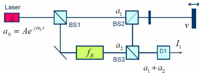
Figure 1: The modules of the Laser Doppler Vibrometer (LDV)
