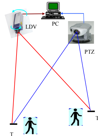
Figure 2: Schematic setup of the remote audio/video acquisition sensor system
