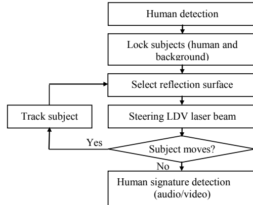
Figure 4: Flow chart of video analysis
