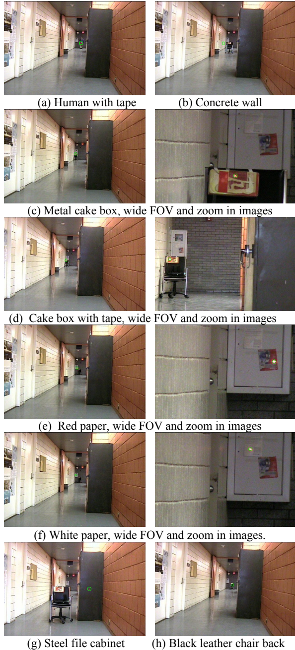
Figure 6: Various reflection surface experiments (The laser spot is within a green circle in each image)
